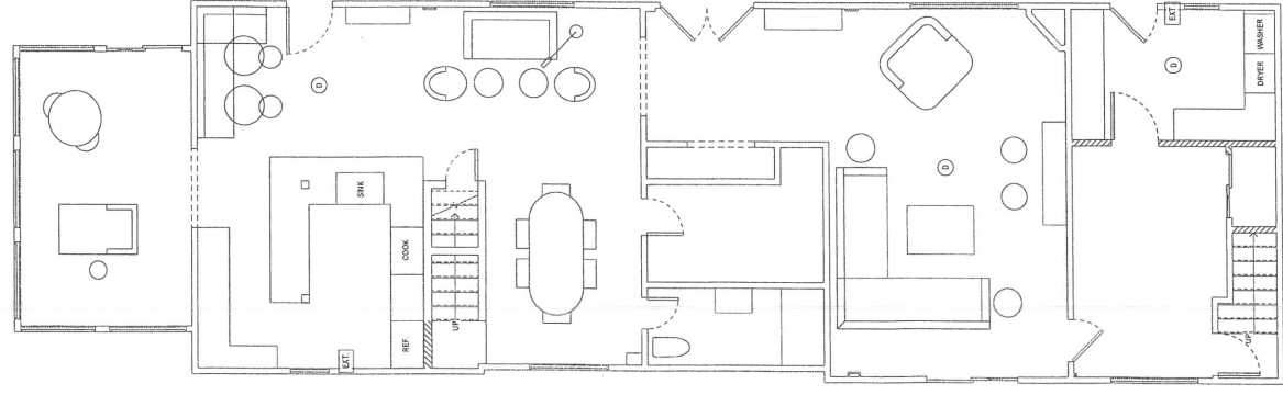
1 FIRST FLOOR PROPOSED PLAN 1/4" = 1'-0"
